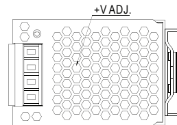
Terminal Pin No. Assignment (TB1)
